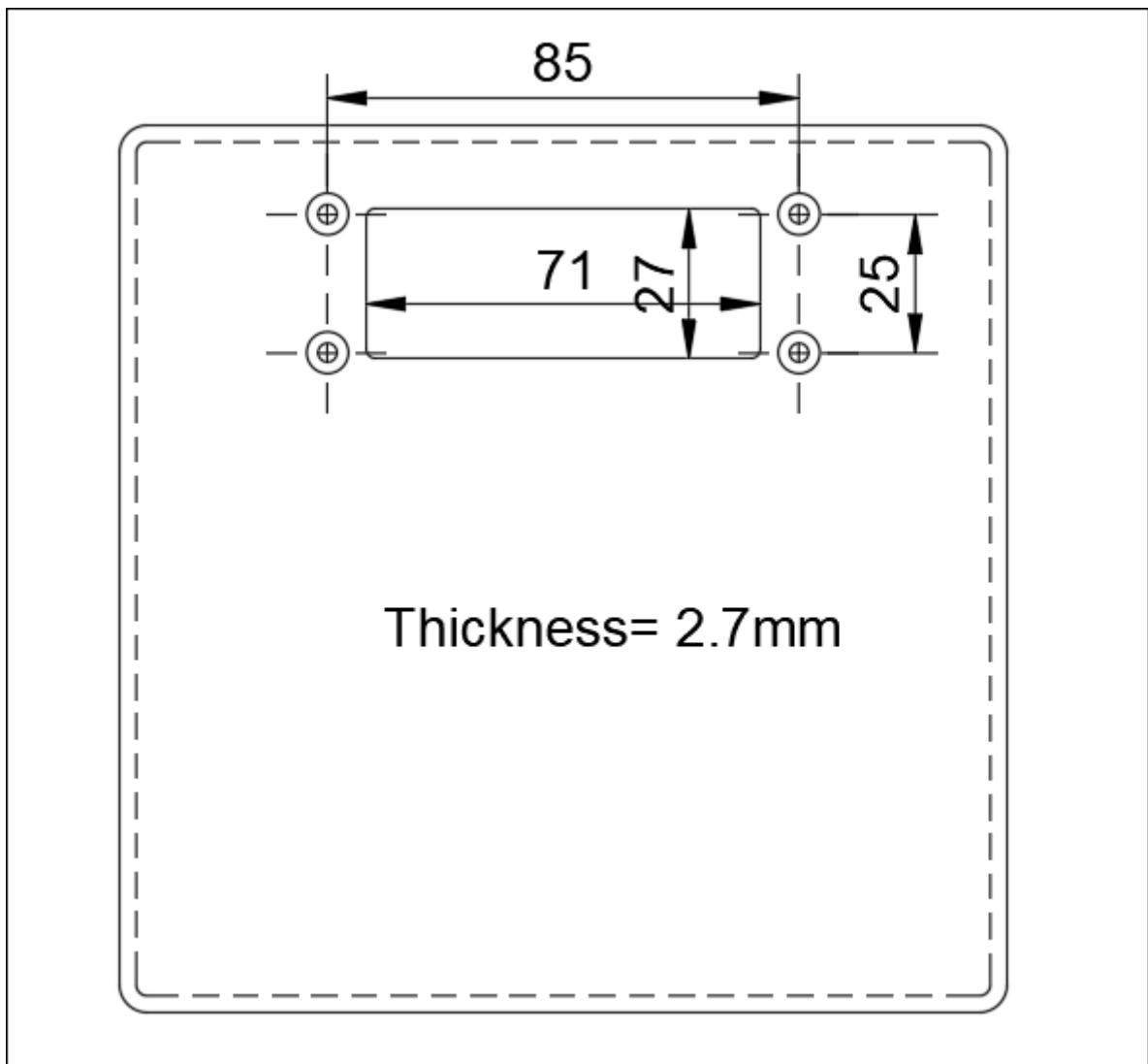
Part drawing
